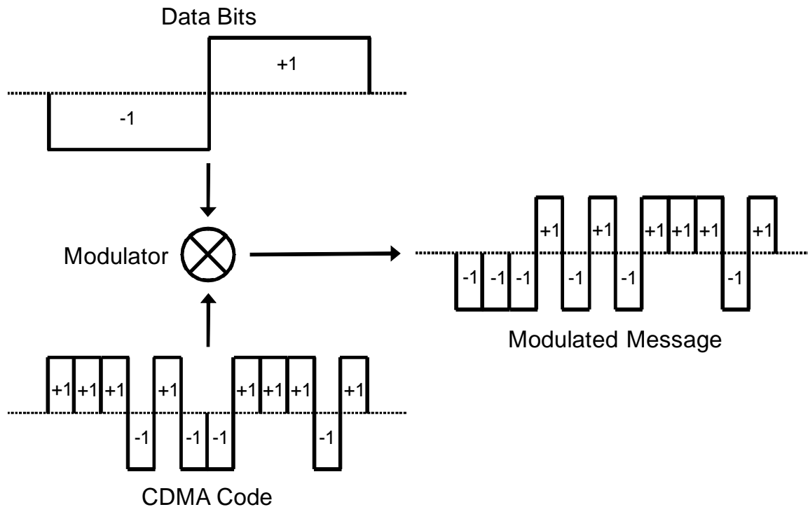
Figure 4-16: Example of DS-SS-SSA Modulation
