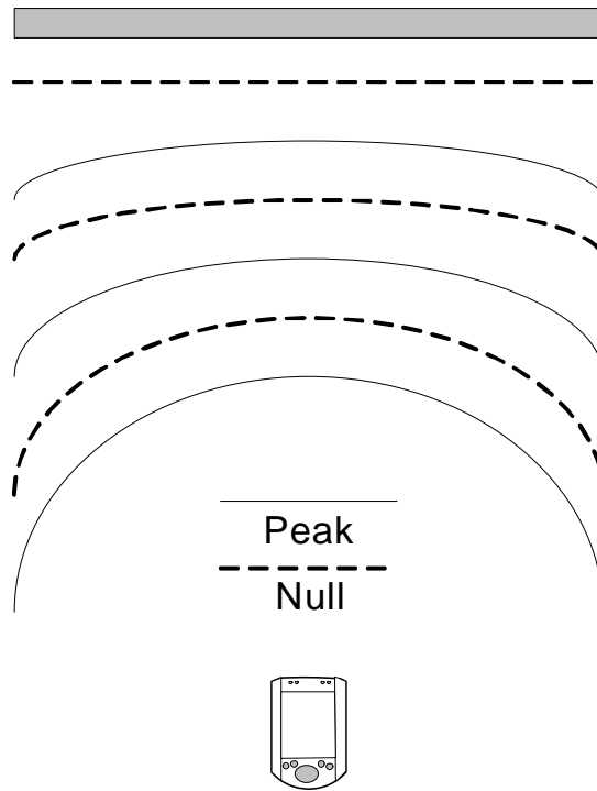
Figure 4-7: RF Standing Wave Pattern from a Reflecting Wall 3
