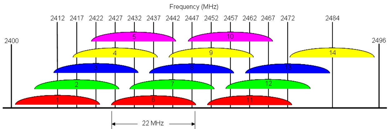
Figure 5-10: IEEE 802.11b/g Channel Allocations
