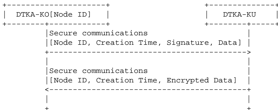
Figure 9: Interaction Diagram 3: Secure communication
