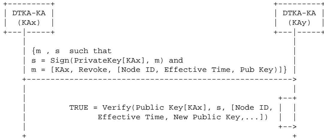
Figure 6: Interaction Diagram 1.1: Key Revocation
