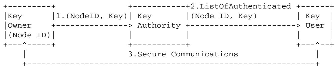
Figure 1: Abstract Data-Flow-Diagram for DTKA
