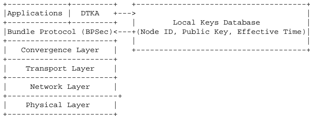
Figure 10: Interaction Diagram 3: Secure communication
