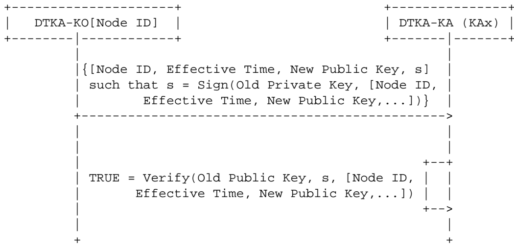
Figure 7: Interaction Diagram 1.2: Key Rollover
