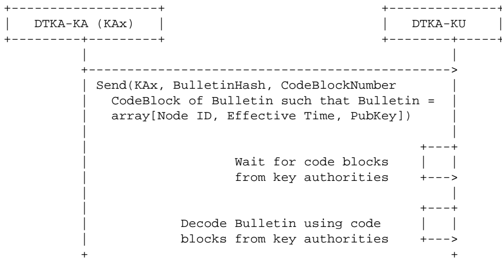
Figure 8: Interaction Diagram 2: Bulk Key Distribution
