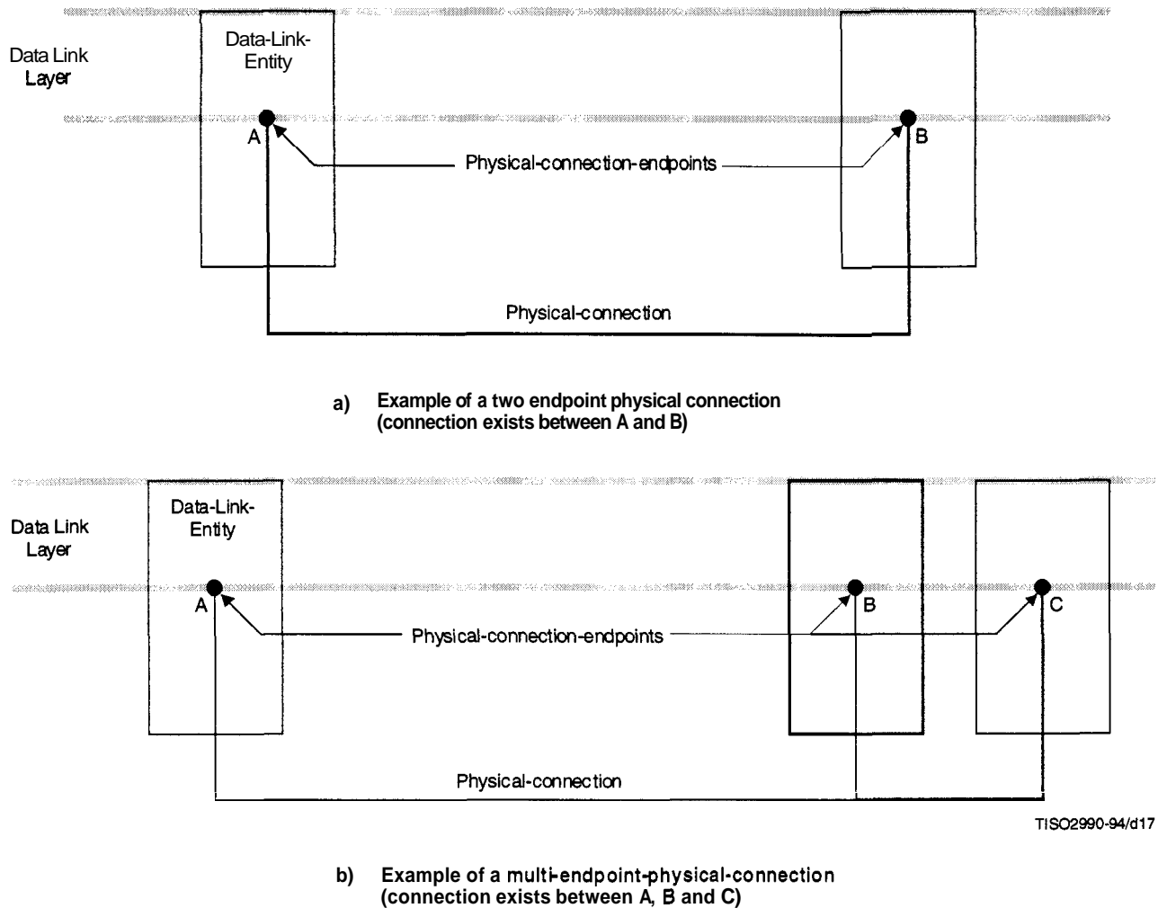
Figure 18 - Examples of physical connections
