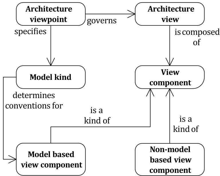
Figure 3 — Conceptual model for views and view components
