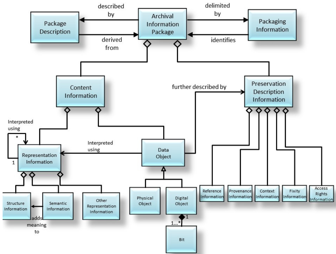
Figure 4-18: Archival Information Package (Detailed View) and its associated Package Description and Packaging Information
