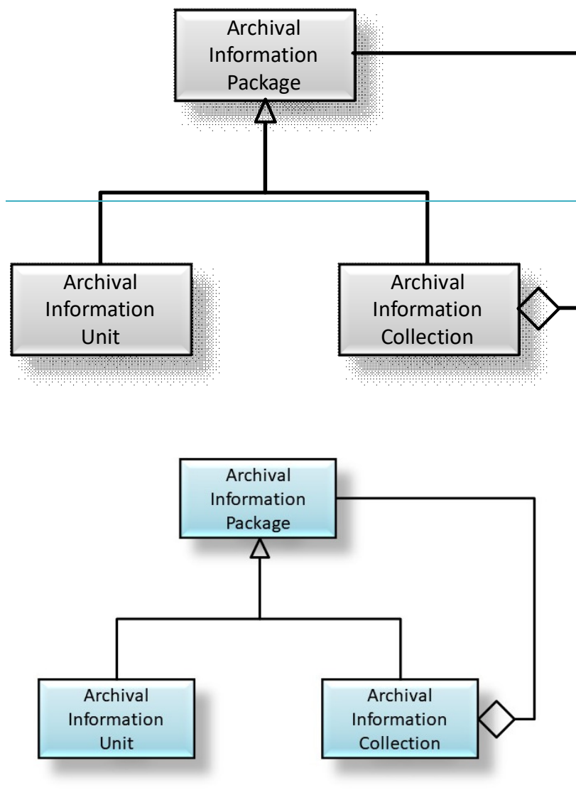
Figure 44-1919: Archival Specialization of the AIP
