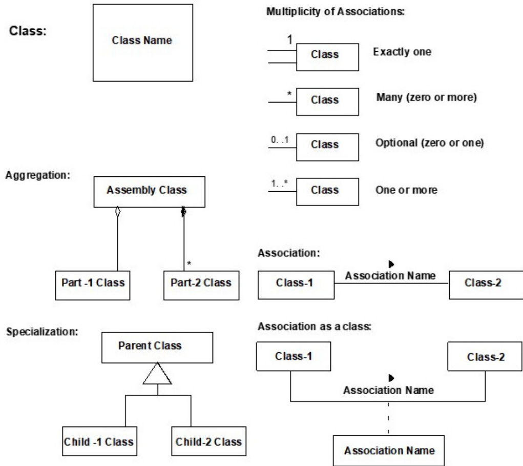
Figure 6-8: -Key to UML Relationships
