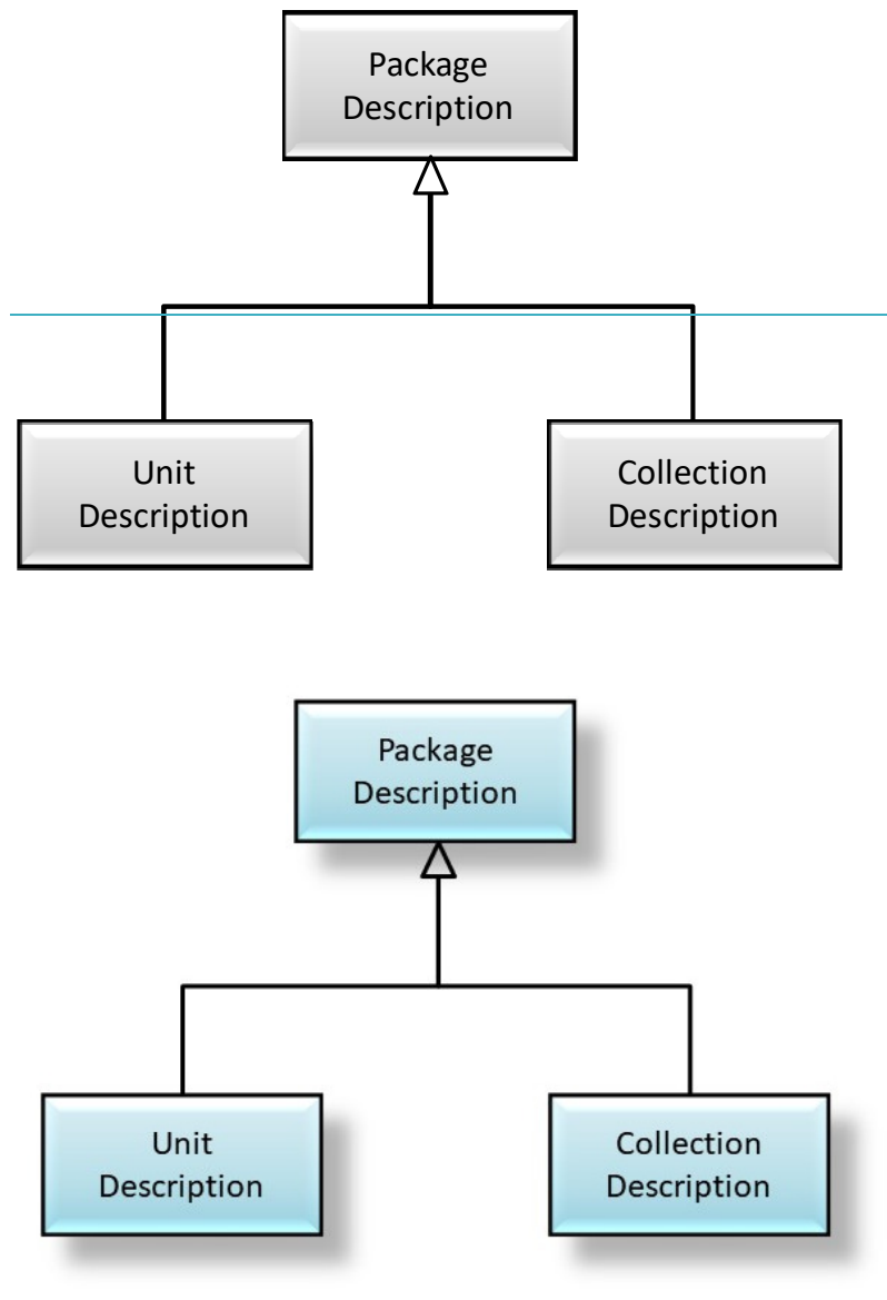
Figure 44-20: Archival 20 : Specialization of the Package Description
