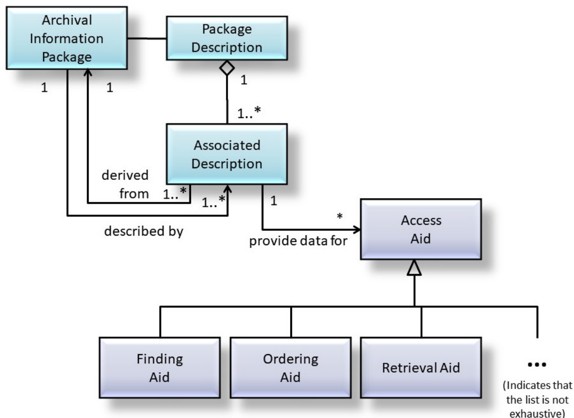
Figure 4-17: Package Description and its associated AIP
