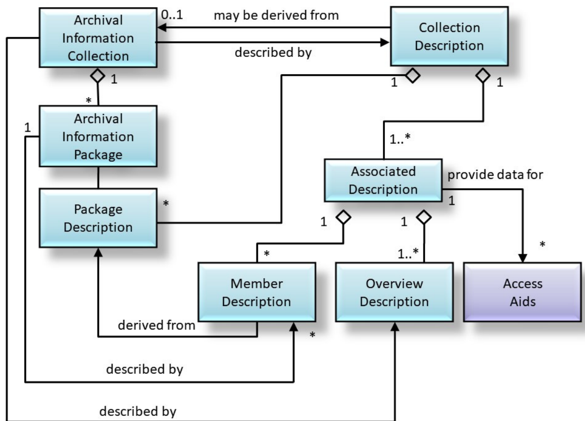
Figure 4-24: Collection Description and its associated Archival Information Collection
