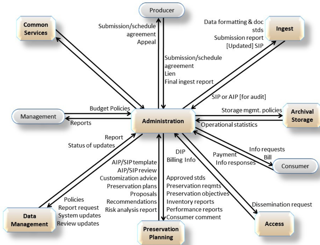
Figure 4-9: -Administration Context Diagram
