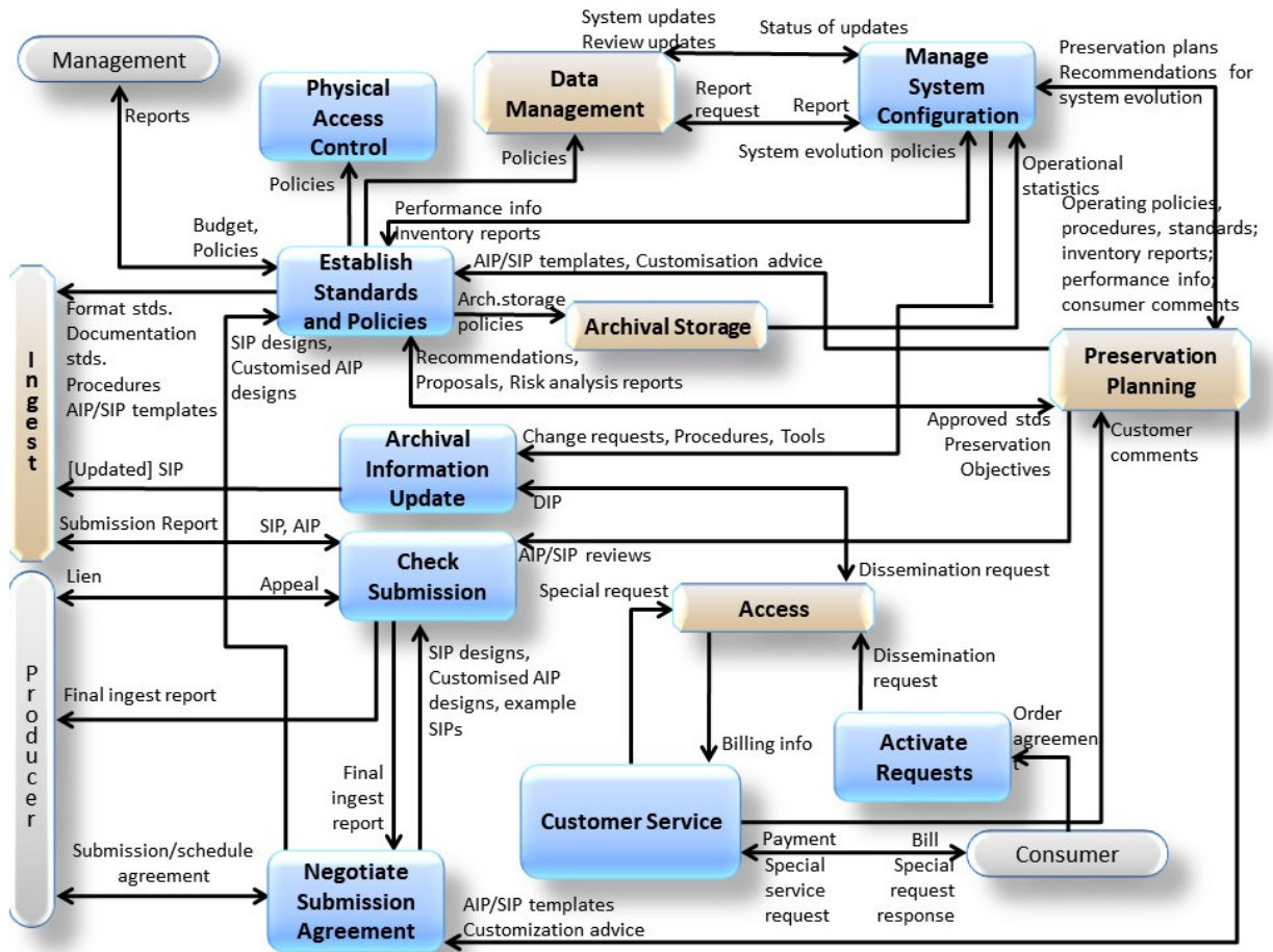
Figure 4-5: Functions of the Administration Functional Entity
