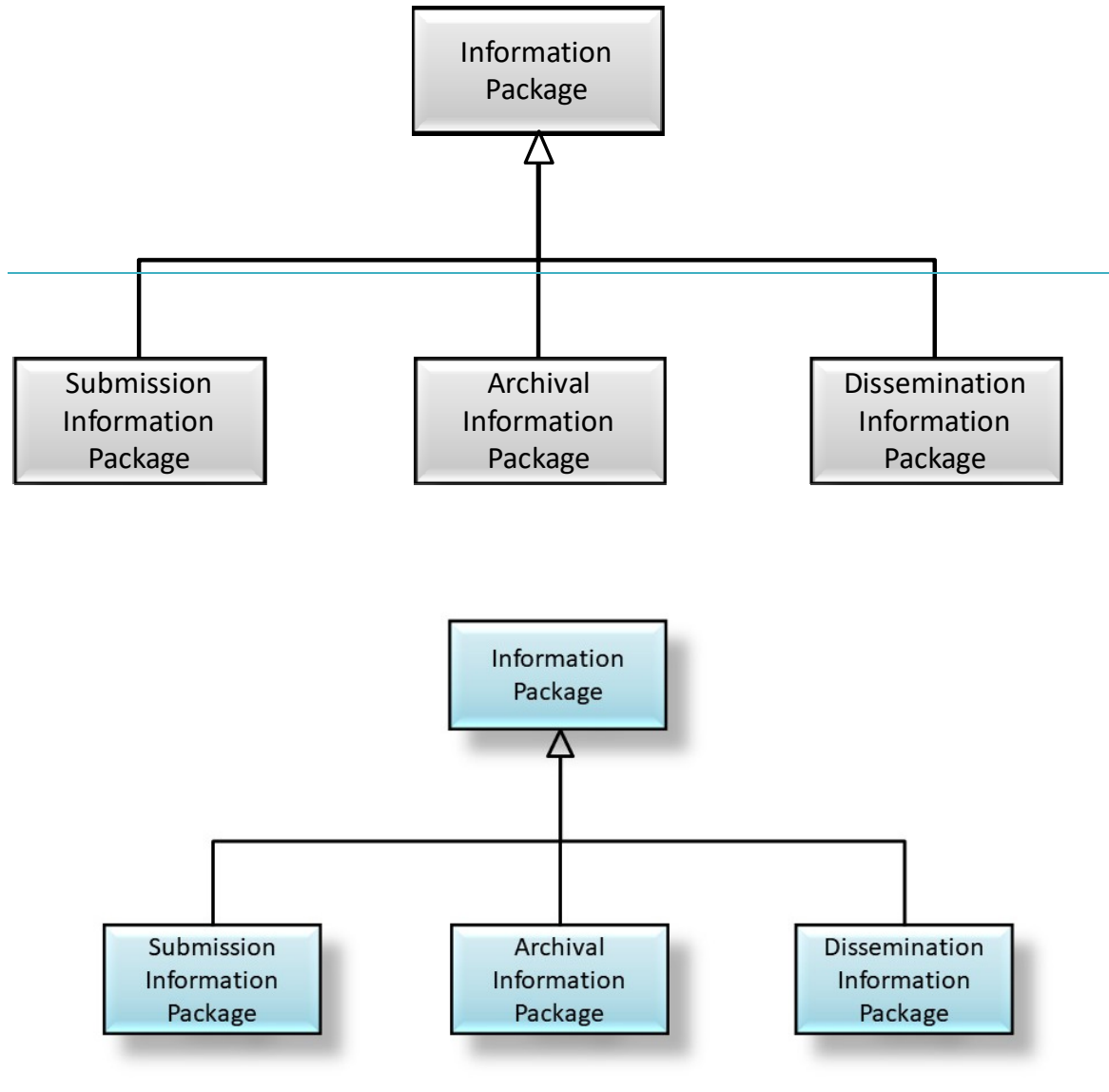
Figure 44-1414: Information Package Taxonomy
