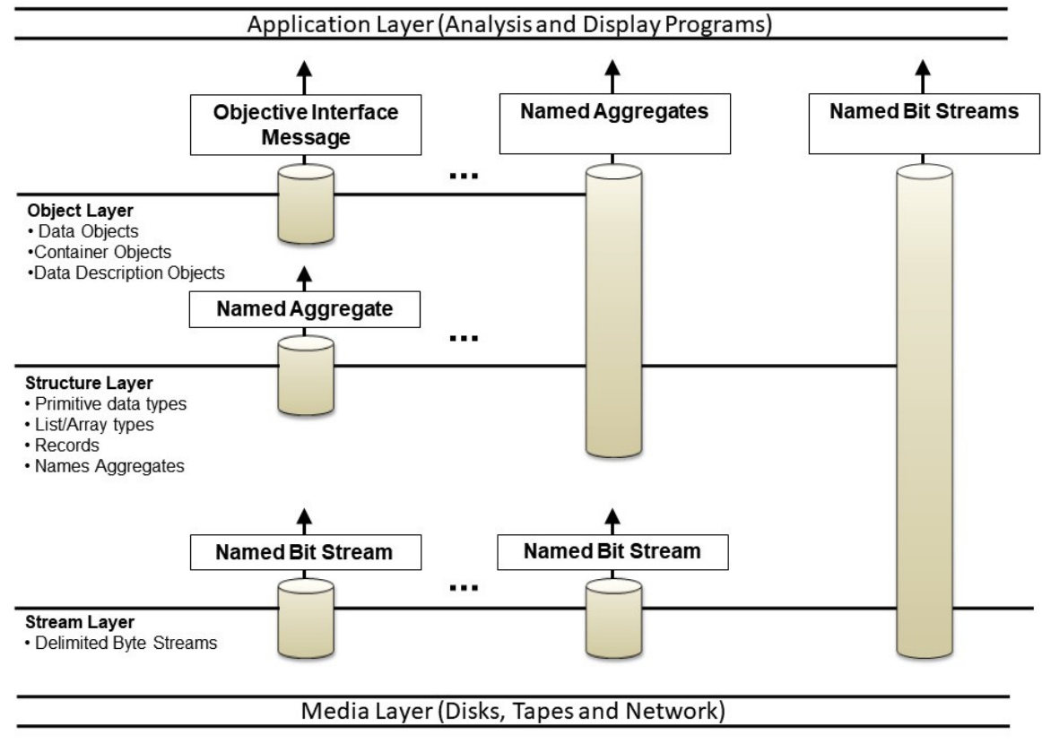
Figure E6-19: Layered Information Model
