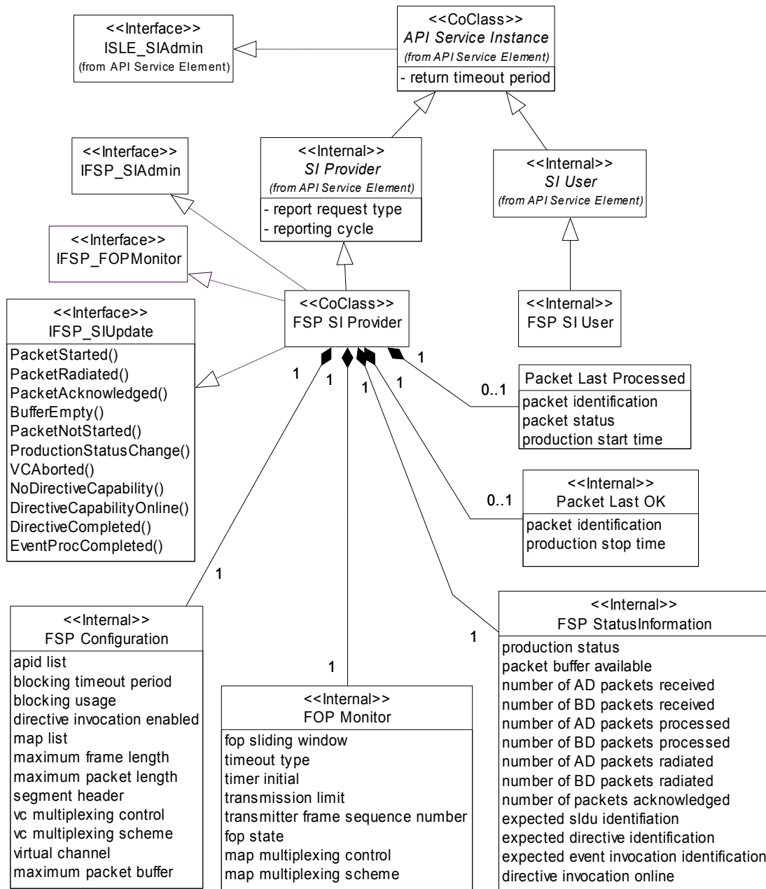
Figure 2-1: FSP Service Instances
