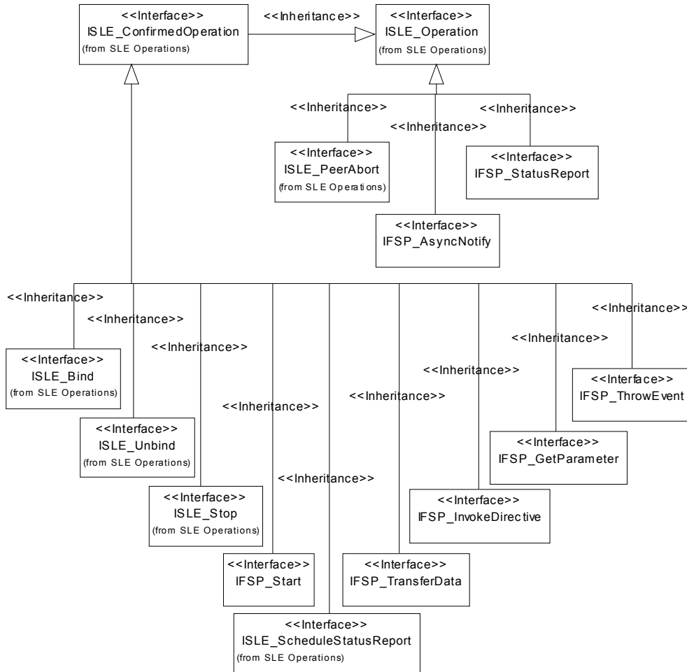
Figure 2-2: FSP Operation Objects
